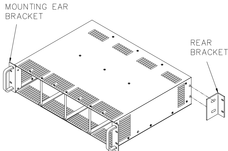
FIGURE 1. RA 61 RACK ADAPTER ASSEMBLY
